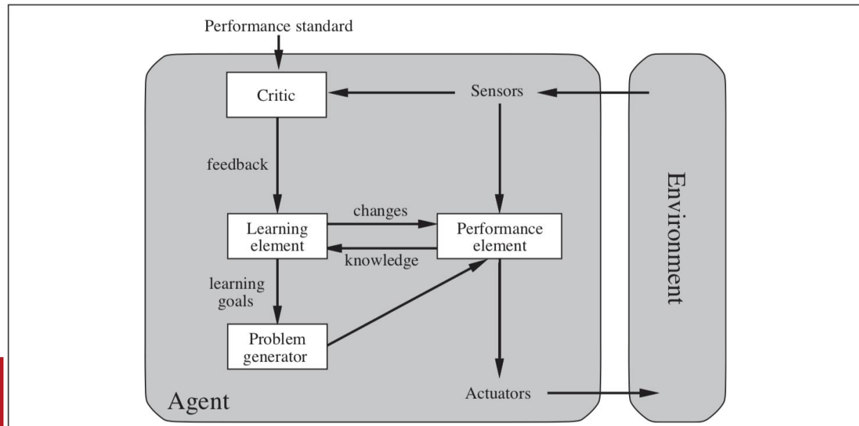
Figure 2.15 A general learning agent.
